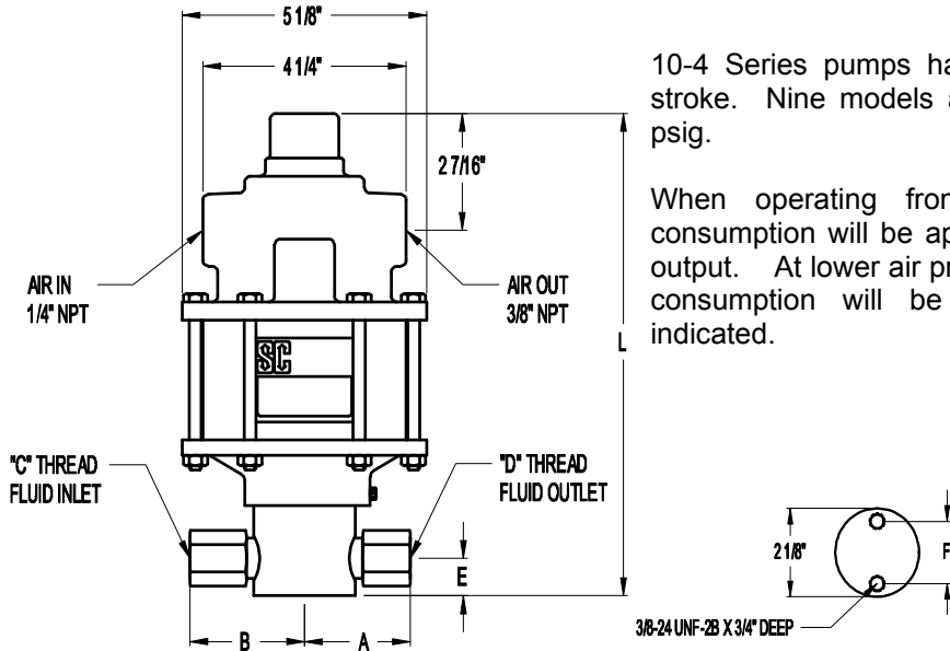
Mounting Dimensions in Inches
