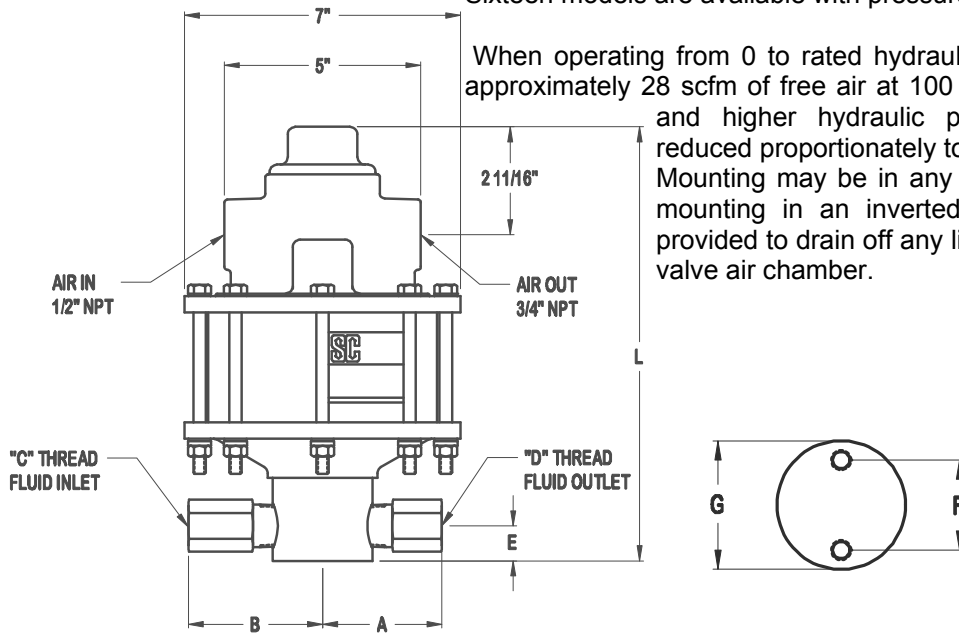
Mounting Dimensions in Inches
